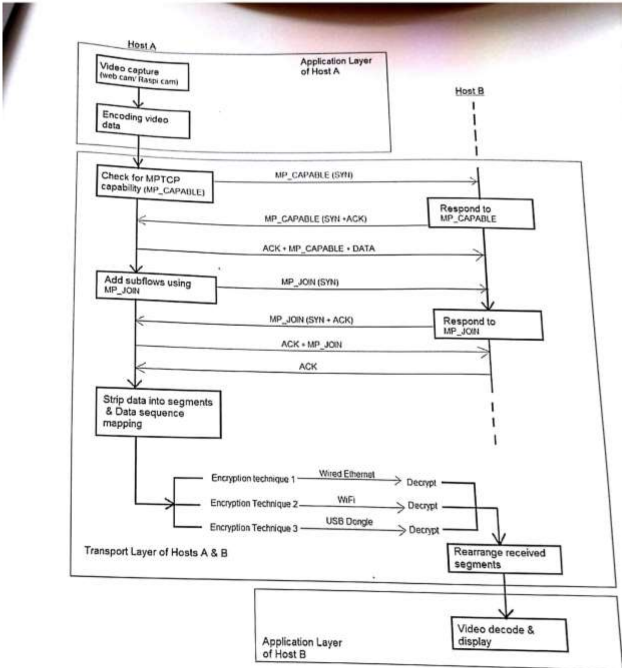
Figure 1: Flow of Implementation of Multipath TCP for Video Streaming
