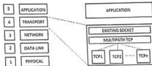
Figure 2: MPTCP in Transport Layer of TCP/IP model
