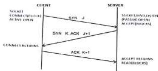
Figure 3: TCP Three Way Handshaking
