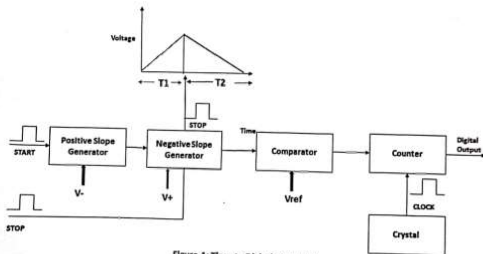
Figure 1: Time to Digital Converter
