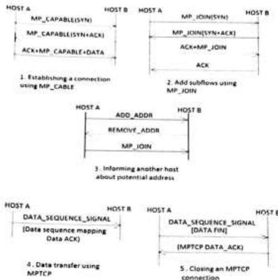
Figure 4: MPTCP Handshaking and Data Transfer
